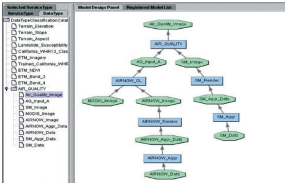
Analyst creates a new image by 'chaining' services from multiple sources.
