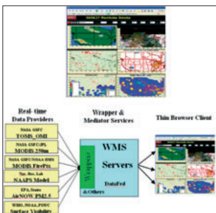
Data from many sources can be automatically accessed and combined.
